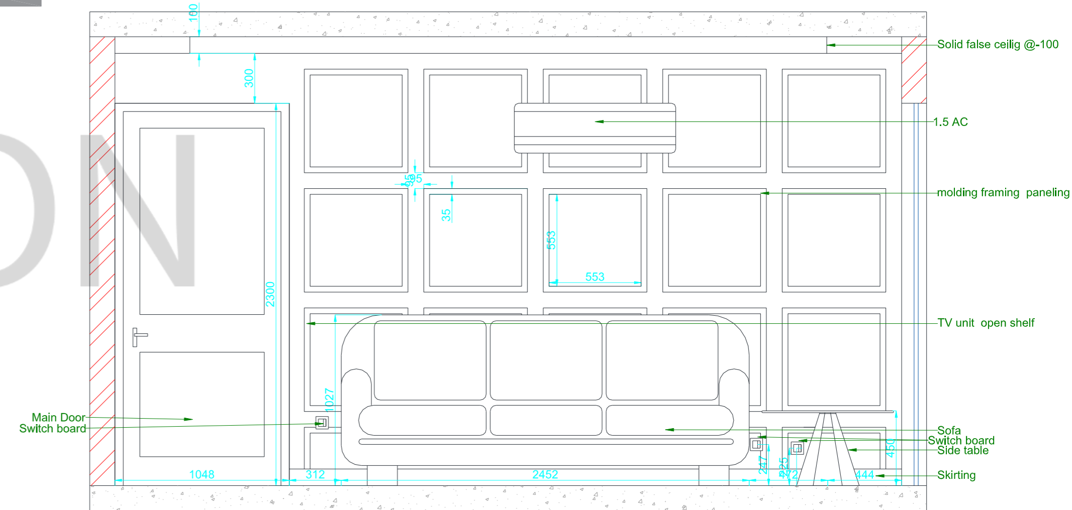
Elevation B detailing of Drawing And Dining Area
