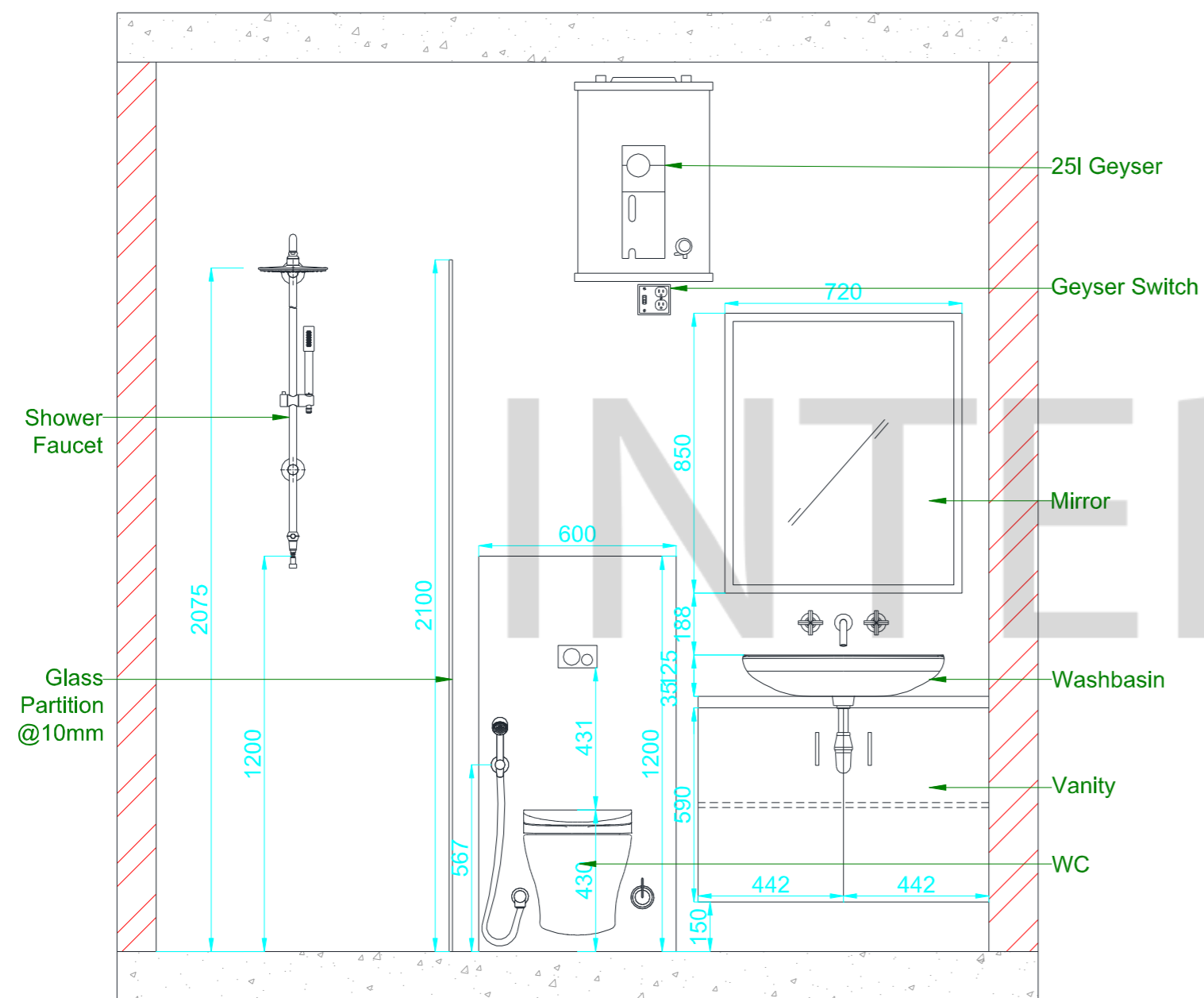
Elevation C detailing of Bathroom_1
